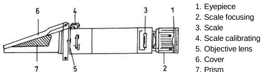
Hand refractometer
