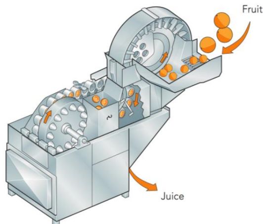
Orange RTS extraction (Reamer type)
